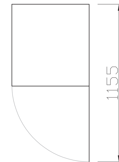
Schema of opening (scale 1:20)
